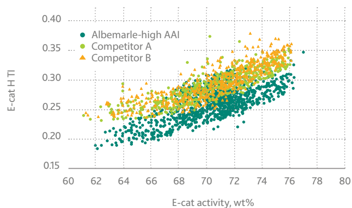
Figure 2: AFX catalysts reduce hydrogen transfer reactions by employing Albemarle’s high accessibility technology
