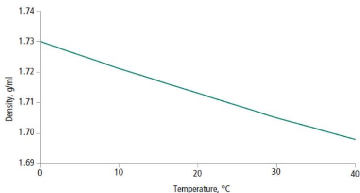
Variation of the density of WELLBROM 14.2 with temperature
